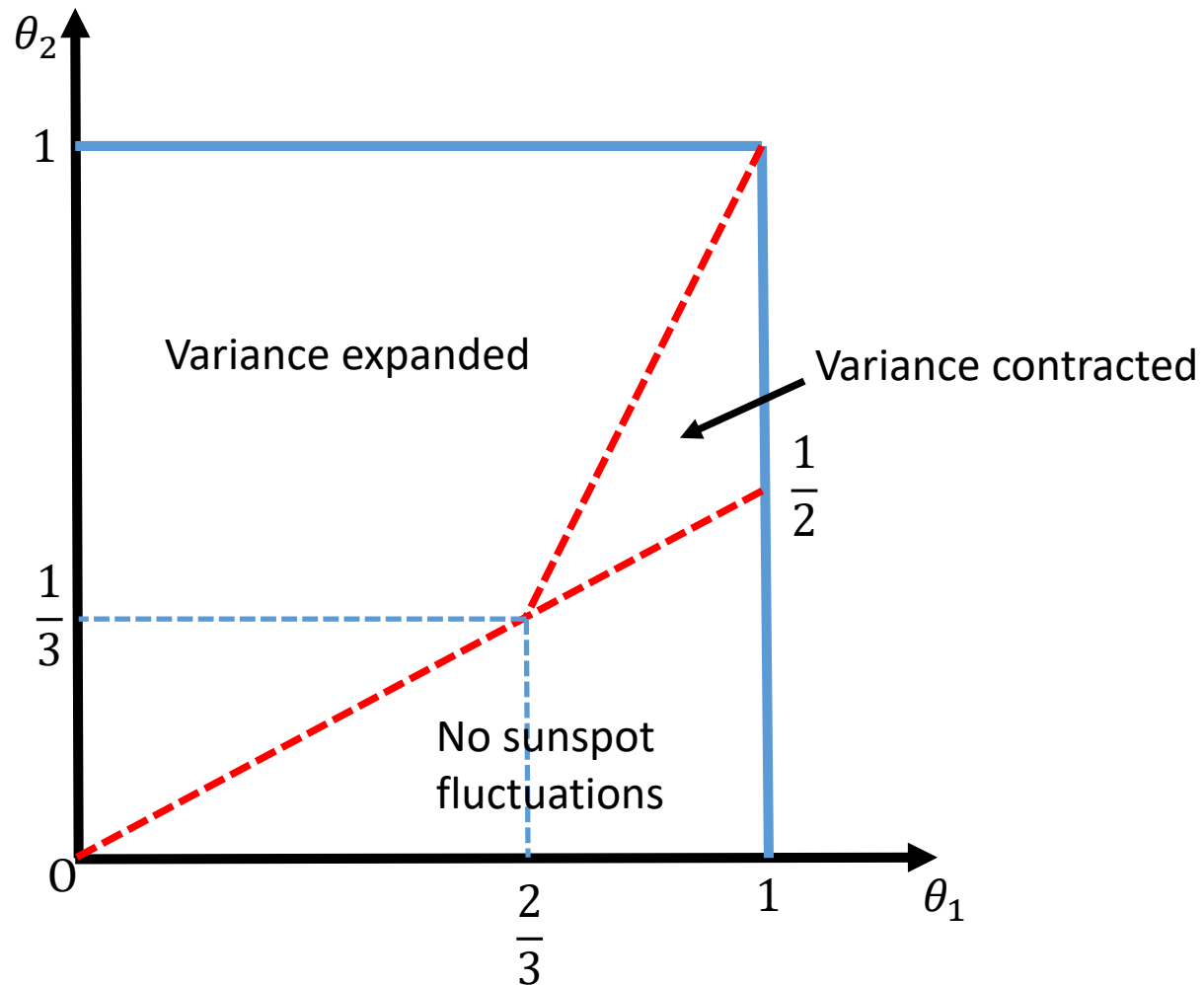
Fig. 1: The effect of financial development on the gross product variance. Notes: In the variance-expanded region, the variance of the gross product is expanded as \mu increases, whereas in the variance-contracted region, the variance of the gross product is contracted as \mu increases.
