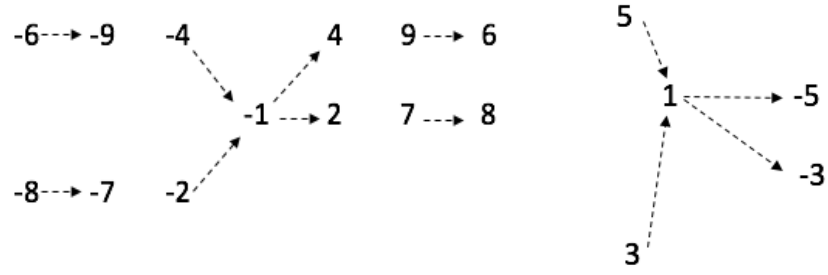
Figure 1: \succsim^R at \xi = 0
